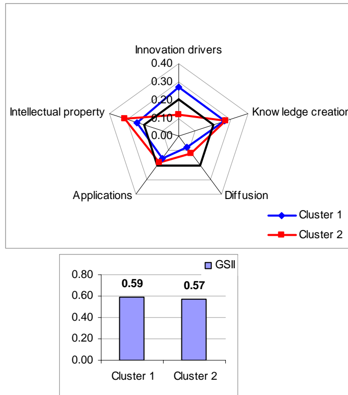
FIGURE 9: CLUSTER GROUPINGS
